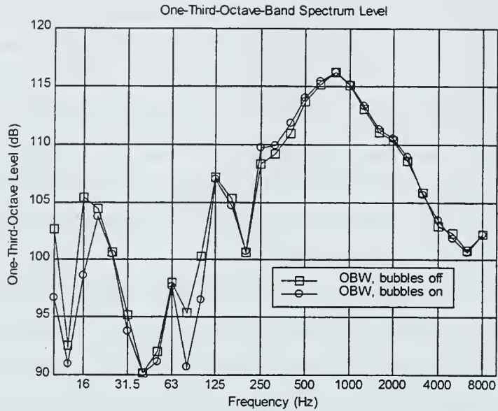
Figure 5.2. Observed one-third-octave-band noise spectra versus frequency for the two primary operating conditions of the OBW Exhibit.
